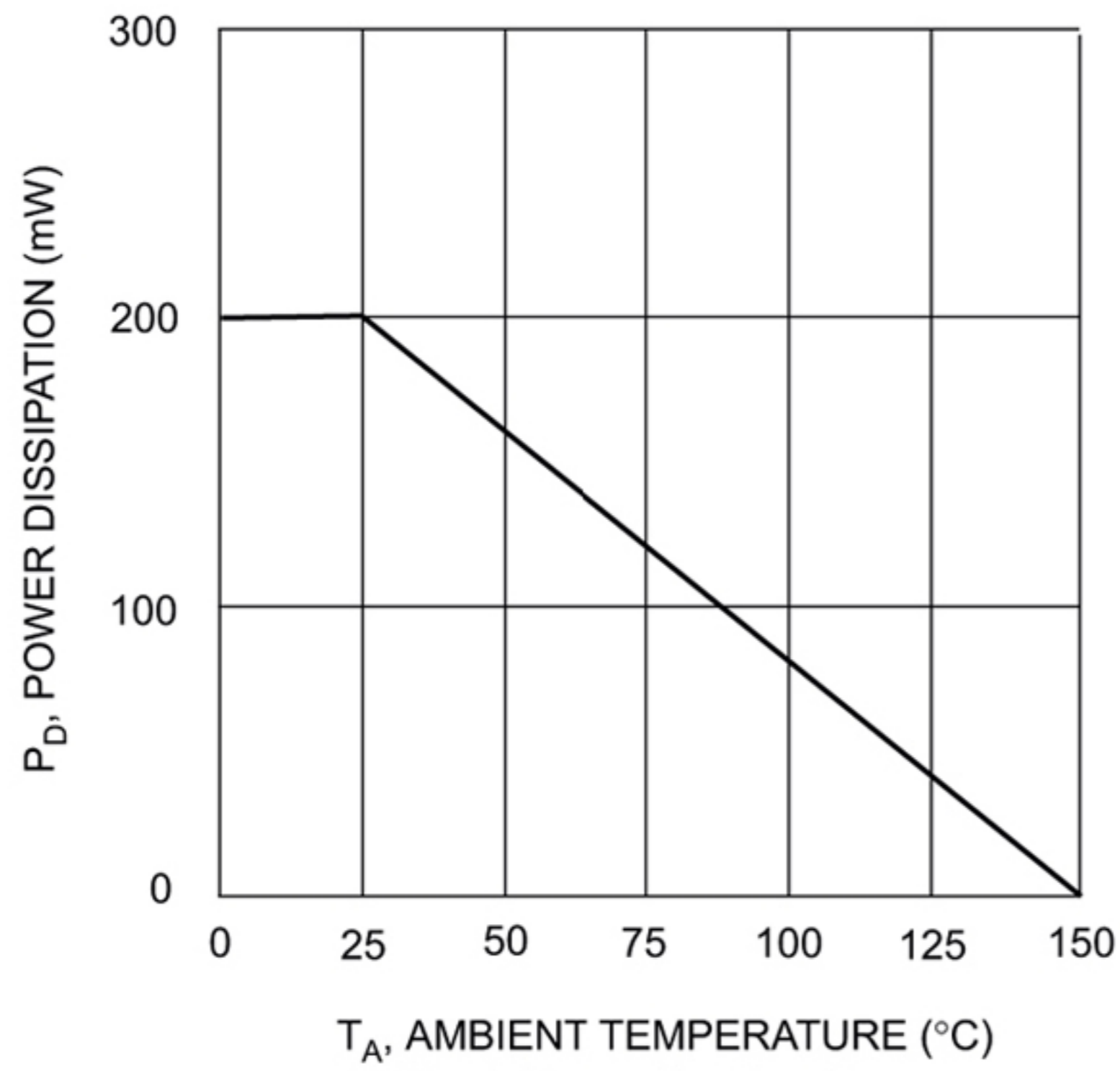
Fig. 1 Power Derating Curve
