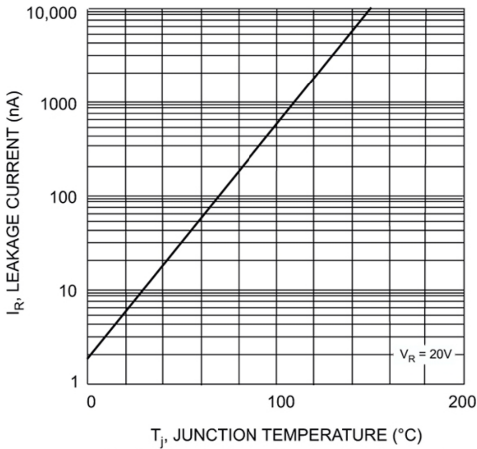
Fig. 3 Leakage Current vs. Junction Temperature
