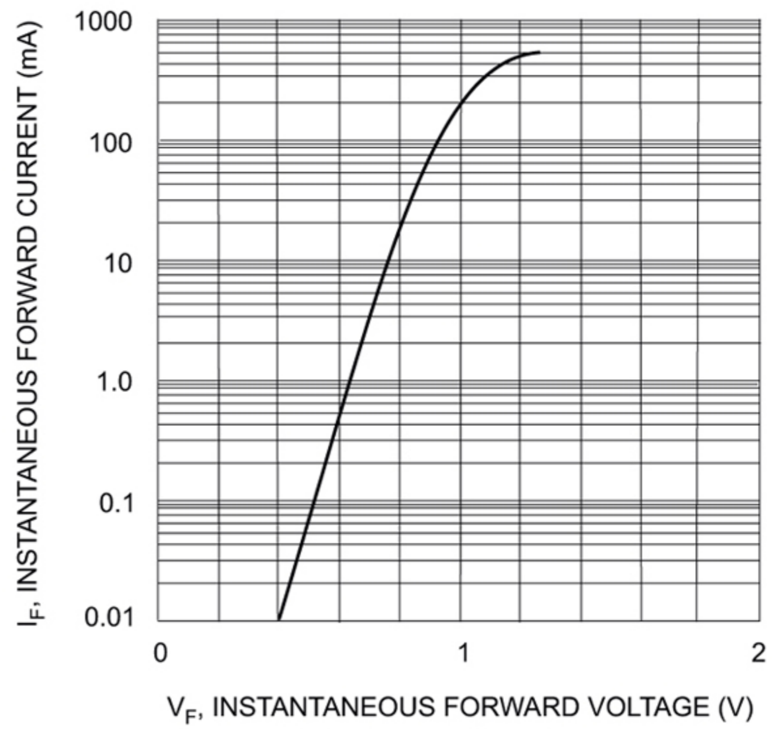
Fig. 2 Forward Characteristics
